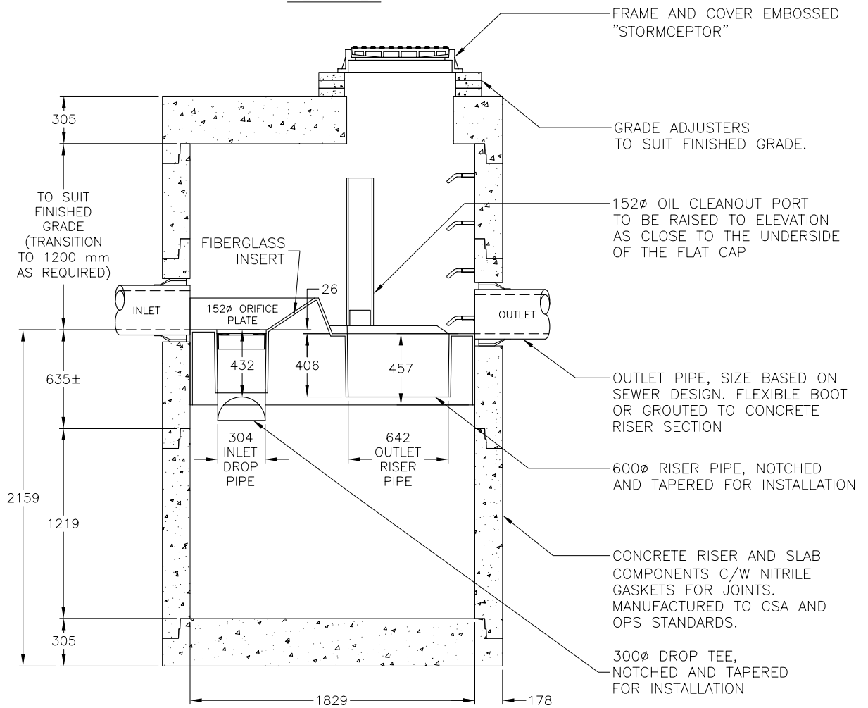
SECTION VIEW
