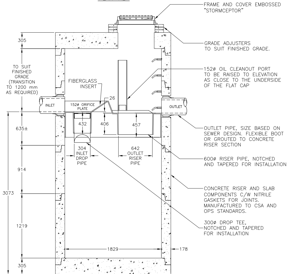
SECTION VIEW
