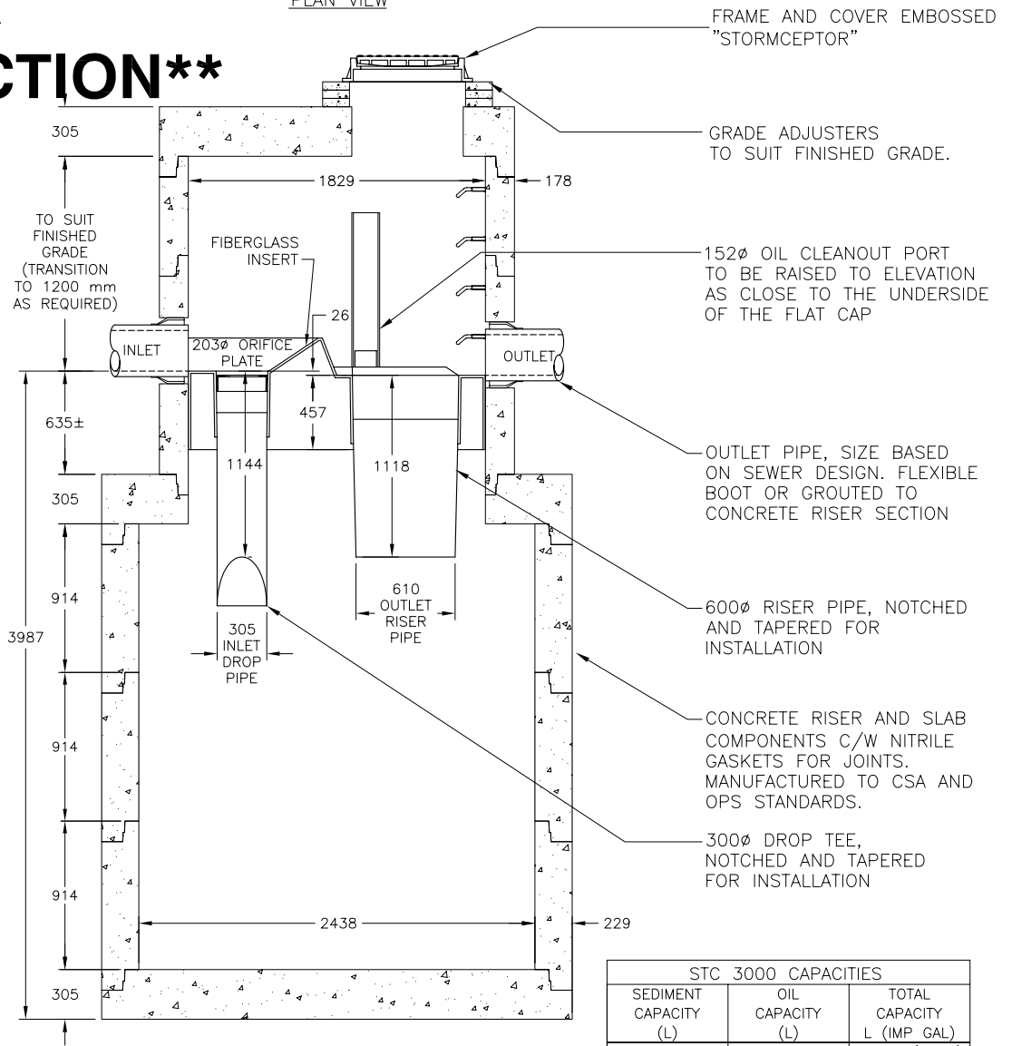
SECTION VIEW
