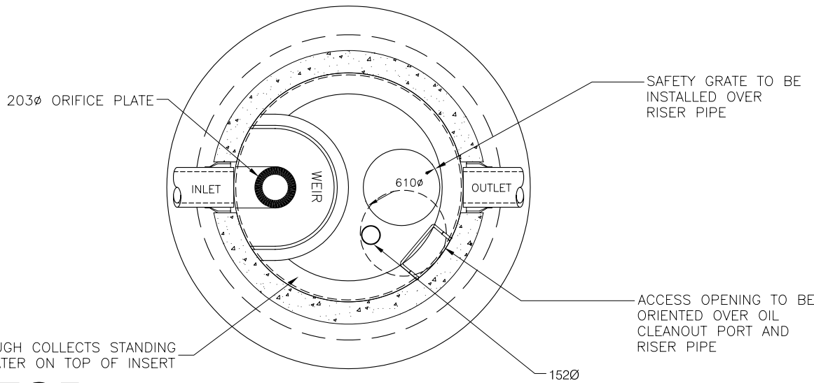
PLAN VIEW
