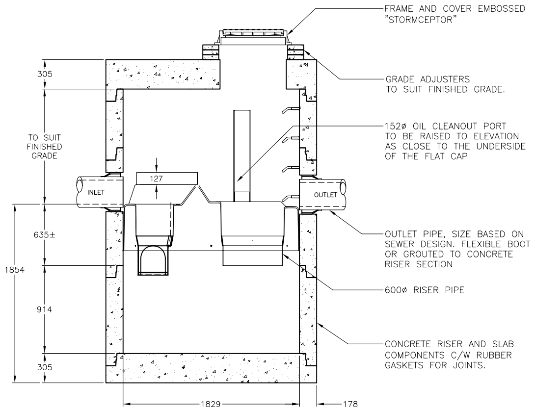
SECTION VIEW
