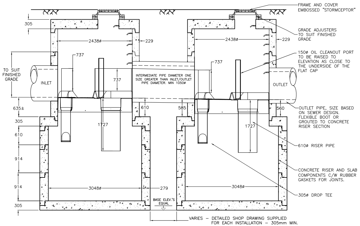
SECTION VIEW
